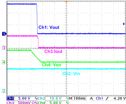
使能关闭 (HT7463A, I OUT =500mA)
